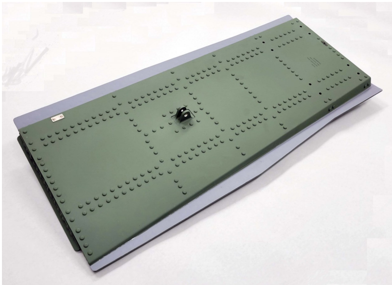
Spot Welded MLG Door Assy Aluminum Size: 2x14x32in Platform: F-15
